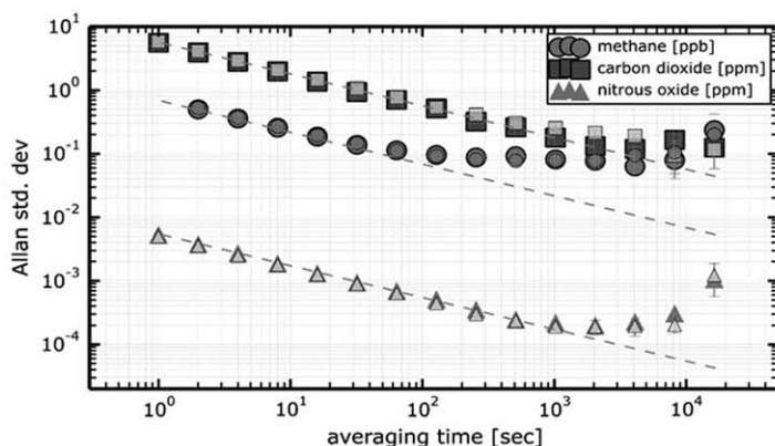
Fig. 1. (A) Allan standard deviation of the Picarro for \text{N}_2\text{O} , \text{CO}_2 , and \text{CH}_4 showing measured data (dark colors) and Monte Carlo modeled data (light colors). The dashed gray lines indicate ideal \tau^{-0.5} averaging of purely Gaussian (white) noise. The error bars indicate the variability of the modeled Allan standard deviation. For most data points, the error bars are smaller than the size of the symbols. (B) Allan standard deviation of the LGR for \text{N}_2\text{O} , showing measured data (dark triangles) and simulated data (gray triangles). The dashed line shows the white noise contribution with a dependence of \tau^{-0.5} , and the dot-dashed line shows the brown noise contribution with a dependence of \tau^{+0.5} .
