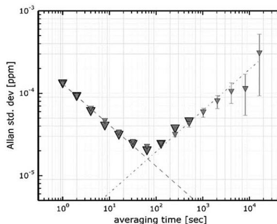
Fig. 1. (A) Allan standard deviation of the Picarro for \text{N}_2\text{O} , \text{CO}_2 , and \text{CH}_4 showing measured data (dark colors) and Monte Carlo modeled data (light colors). The dashed gray lines indicate ideal \tau^{-0.5} averaging of purely Gaussian (white) noise. The error bars indicate the variability of the modeled Allan standard deviation. For most data points, the error bars are smaller than the size of the symbols. (B) Allan standard deviation of the LGR for \text{N}_2\text{O} , showing measured data (dark triangles) and simulated data (gray triangles). The dashed line shows the white noise contribution with a dependence of \tau^{-0.5} , and the dot-dashed line shows the brown noise contribution with a dependence of \tau^{+0.5} .
